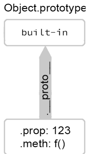
Figure 17.1: Here object literal's __proto__ points to Object.prototype
