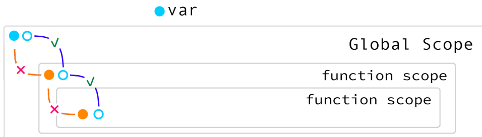
Figure 7.3: Nothing can get out of function scope into its outer scope. This enables the closure pattern. We'll take a look at it in just a moment!
