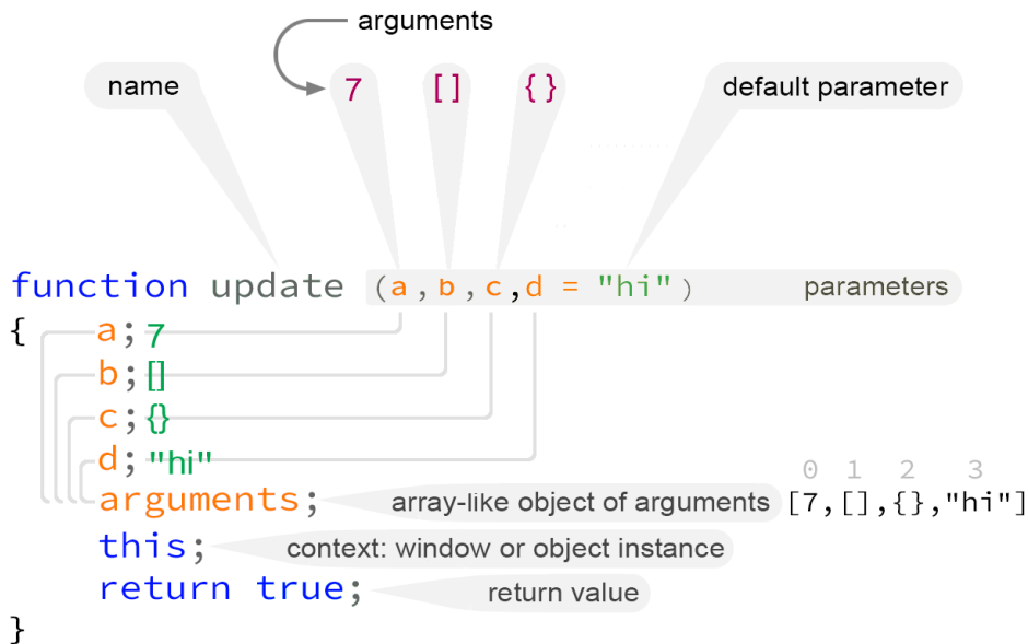
Figure 1.2: JavaScript function anatomy.
