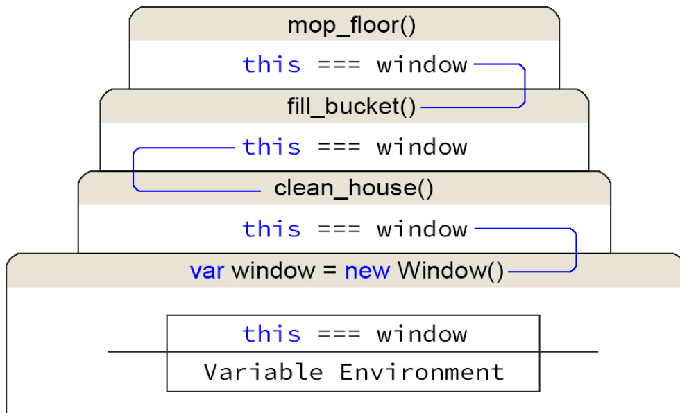
Figure 22.8: As more functions that depend on each other are called from within other functions, the stack grows.
