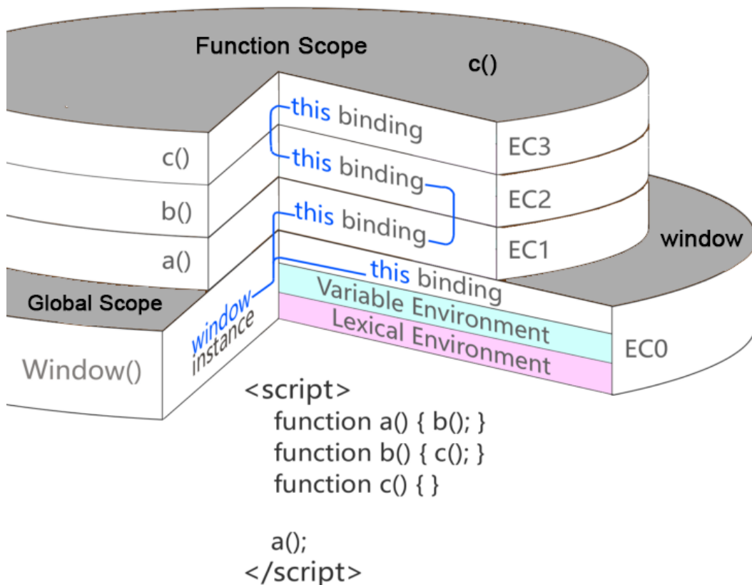
Figure 22.9: Calling multiple functions from within each other's scope will build a tower of function calls on the call stack. Note that this would happen only one at a time for each function if all functions were called from global scope context.
