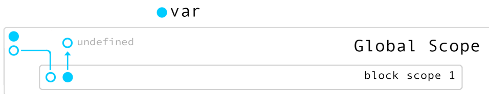
Figure 7.1: Here var is defined in Global Scope, but its value propagates into the block scope as well. What actually happens is, when block scope 1 cannot find var definition in within its own brackets, it looks for it in the parent scope. If it finds it there, it inherits its value.
