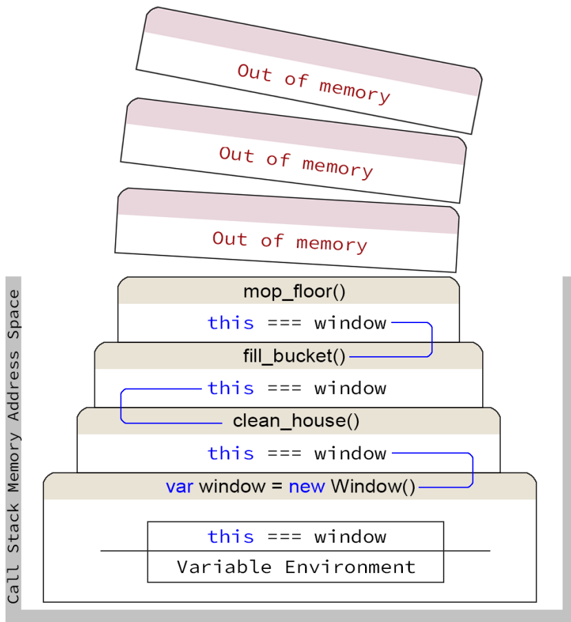
Figure 22.10: Every time a function is called, new context is created in memory. But memory is not infinite. Stack Overflow occurs when the memory required to build the call stack exceeds the address space allocated for the stack. This amount is determined and managed internally by the browser.
