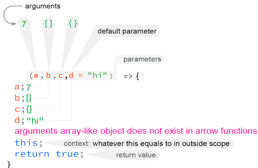
Figure 15.1: Arrow function anatomy.
