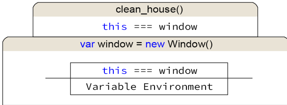
Figure 22.7: Binding of this object across execution contexts on the call stack . A new stack is created when function is called. This new context is logically placed "on top" of the previous object on the call stack.
