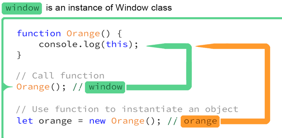
Figure 13.8: This duality of this keyword often causes a headache that you may need to take two Ibuprofens for.
