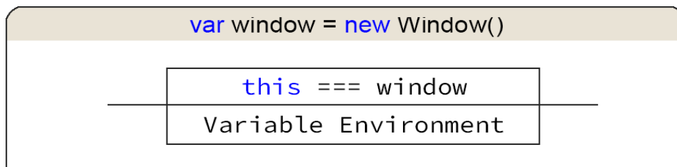
Figure 22.6: A new execution context is created when main window object is instantiated. The this keyword points to the window object.
